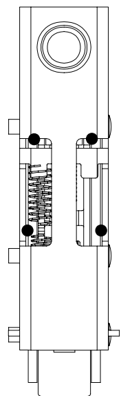
Surface latch, bottom (back of latch)
