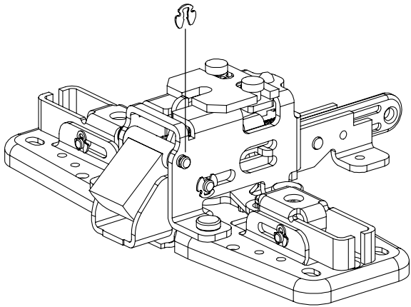
98/99 and 22 rim latch bolt axle (98/99 shown)
