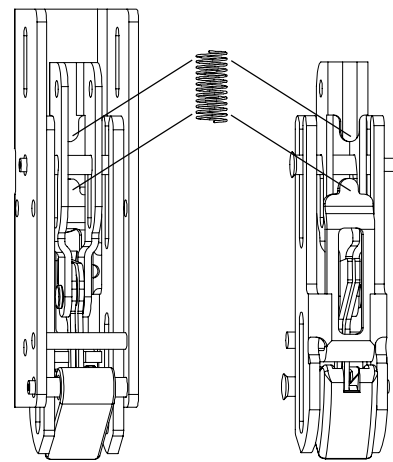
Rear view. Spring fits behind latch bolt axle.
