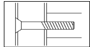
B4 - Single mount on wood or metal door with through bolt.
