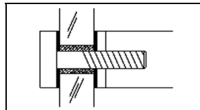
B2 - Single mount on glass door with end cap purchased separately.
